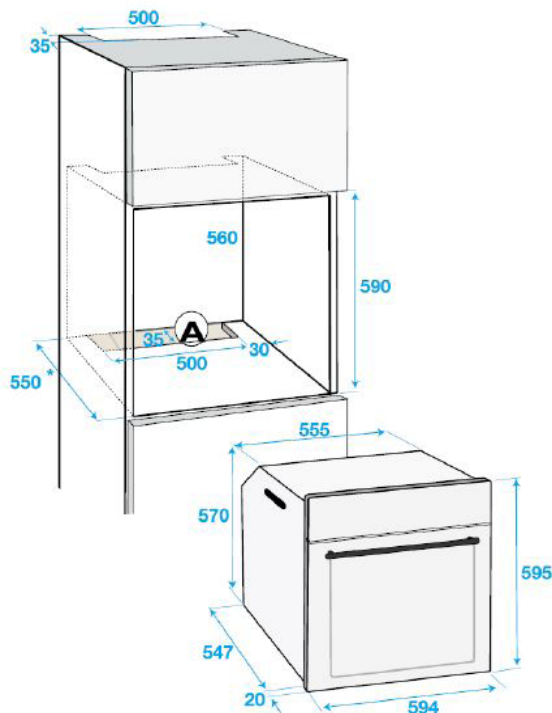
Cabinet Dimensions
