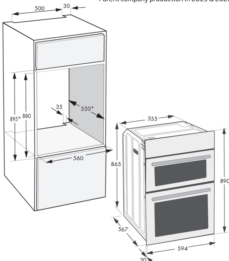
Cabinet Dimensions
