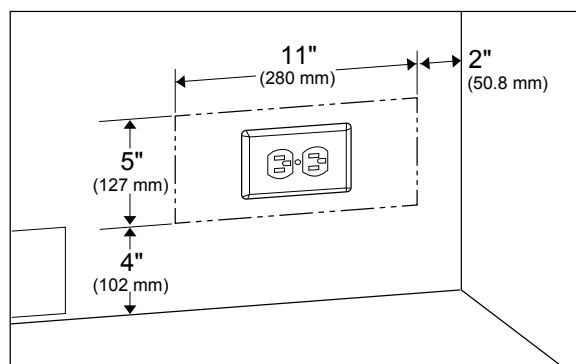
Electrical Location
