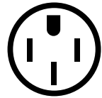
4-wire Wall Receptacle Nema 14-50
