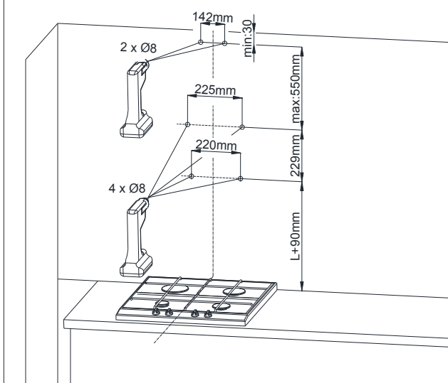
Fig. 4 Installation dimensions.
