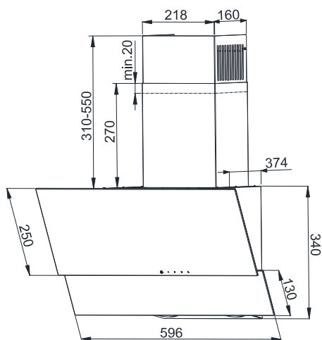
Fig.2 Dimension drawing
