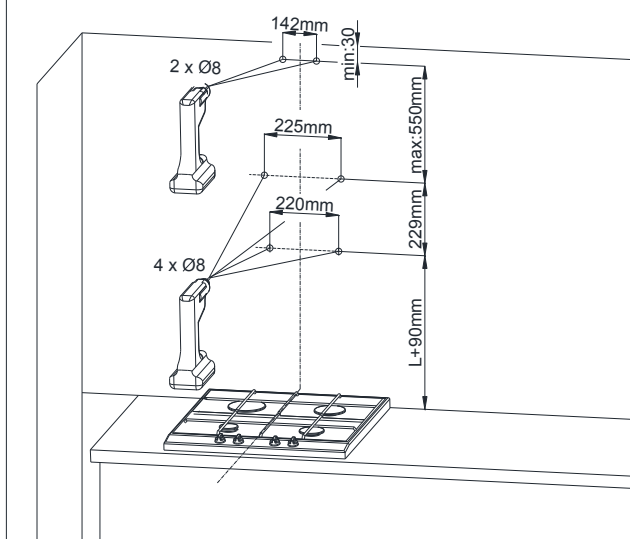
Fig. 4 Instalation dimensions.
