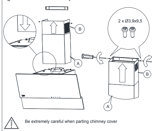
Fig. 9 Hood cover assembly.
