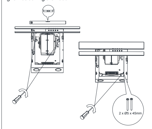
Fig. 8 Positioning the hood.
