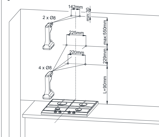
Fig. 4 Installation dimensions.
