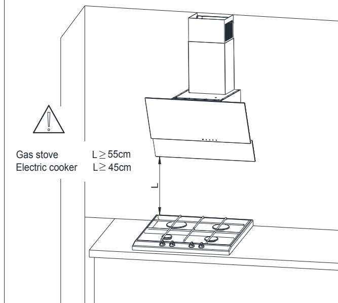
Fig. 3 Suggested distance from the kitchen cooker.
