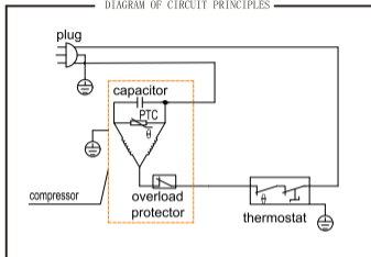
DIAGRAM OF CIRCUIT PRINCIPLES
